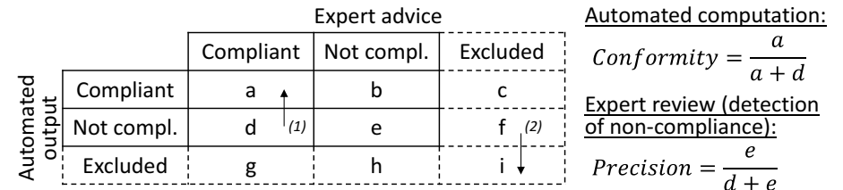
Figure 2. Contingency table of the automated output and the expert advice: conformity rate and precision.
